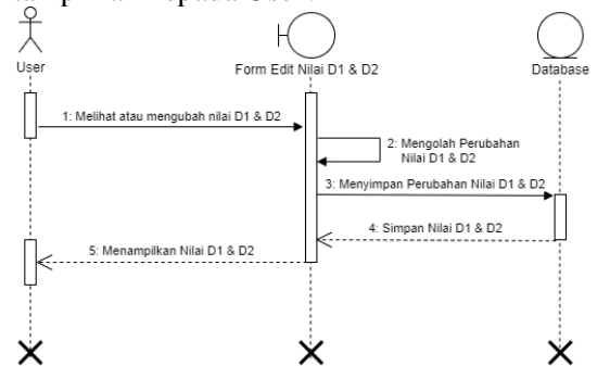
Gambar 5. Sequence Diagram D1 & D2 Sumber: Hasil Pengamatan
