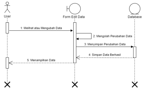
Gambar 4. Sequence Diagram Data Sumber: Hasil Pengamatan
