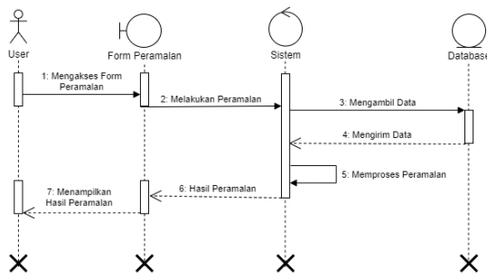
Gambar 6. Sequence Diagram Peramalan Sumber: Hasil Pengamatan
