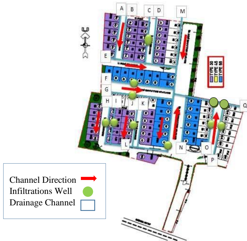
Figure 3. Layout of drainage & infiltration system
