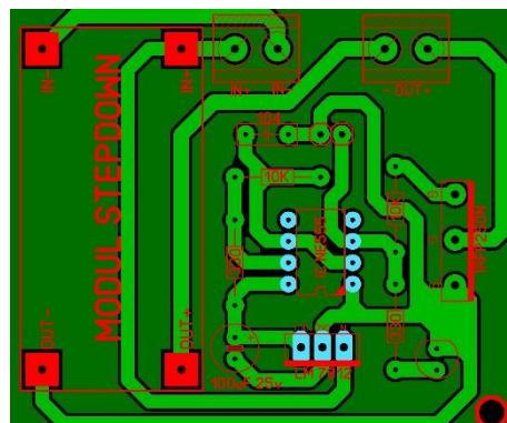
Gambar 3. Desain layout PCB pulsed electric field
