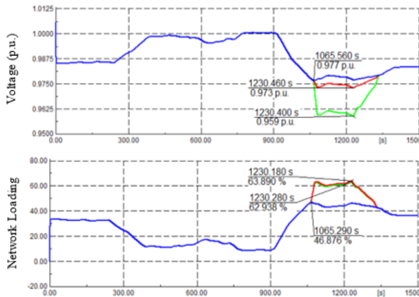
Figure 6. Voltage and feeder loading impact of PEV charging location
