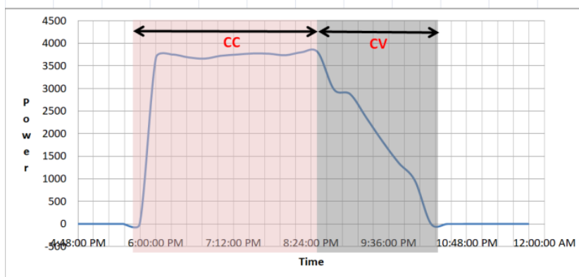
Figure 2. Power profile of PEV charging
