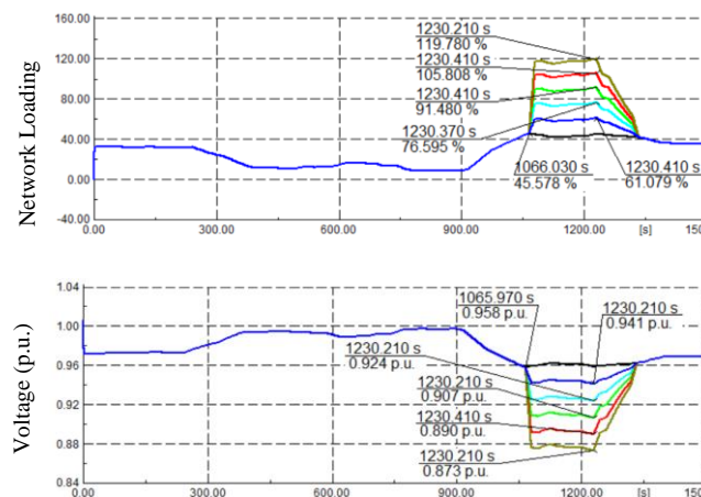
Figure 3. Feeder loading and voltage drop of distribution network model 1
