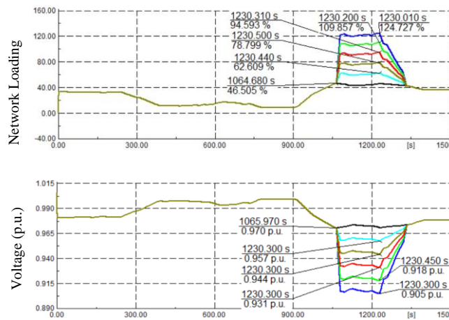
Figure 5. Feeder loading and voltage drop of distribution network model 3
