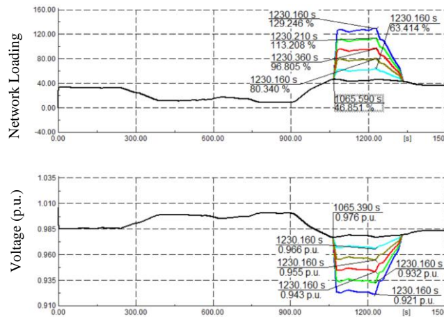
Figure 4. Feeder loading and voltage drop of distribution network model 2
