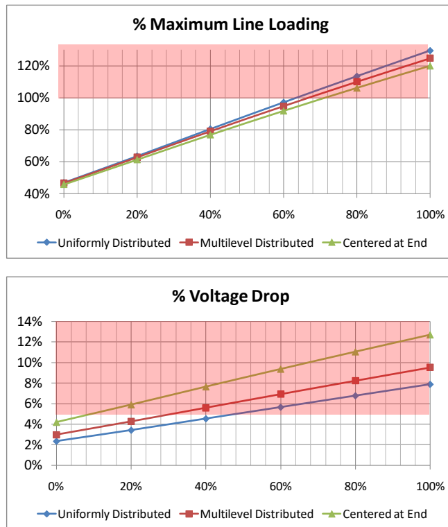
Figure 7. Impact of PEV penetration on maximum line loading and voltage drop
